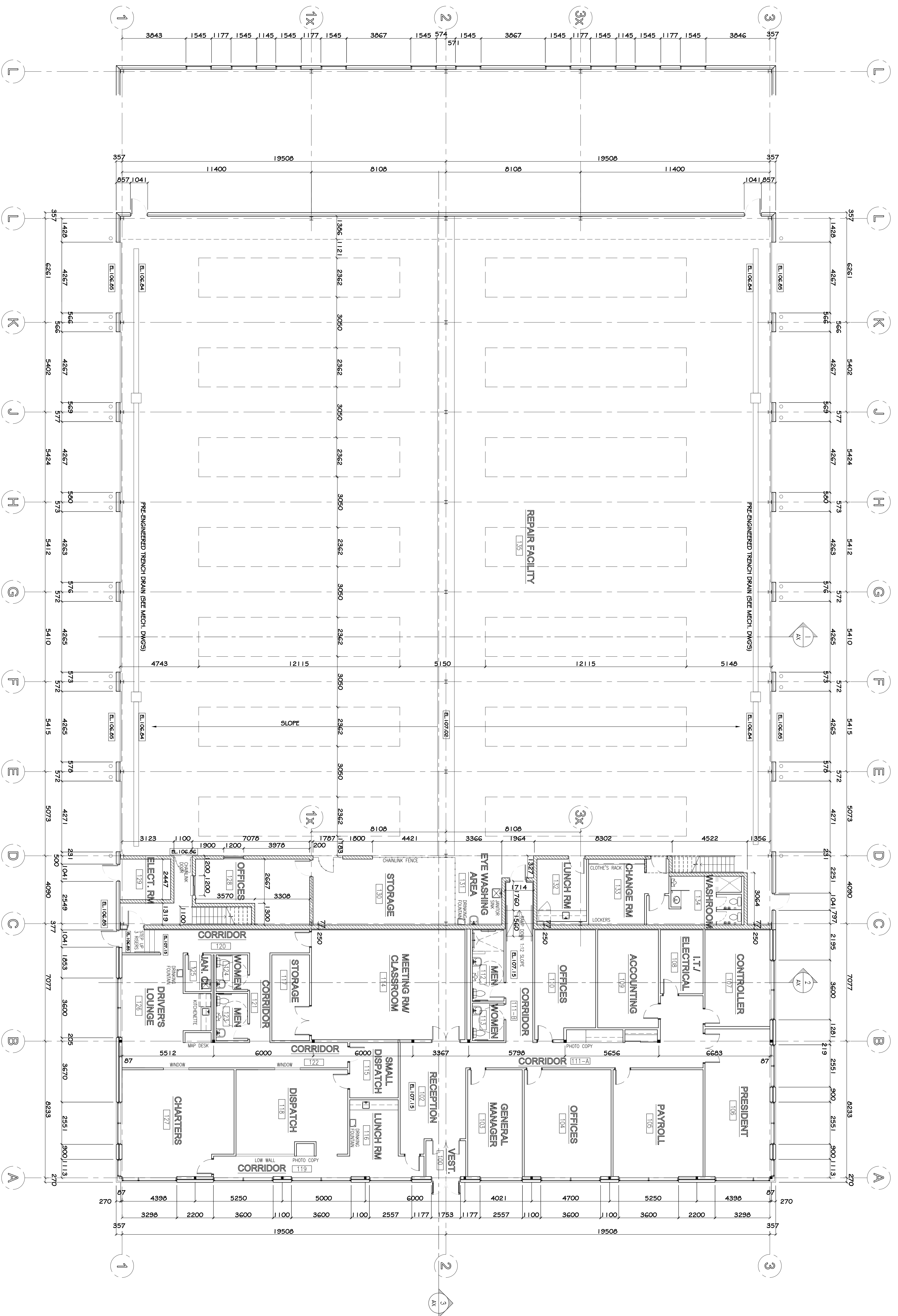
1 GROUND FLOOR PLAN @ WINDOW LEVEL A301 1:100
